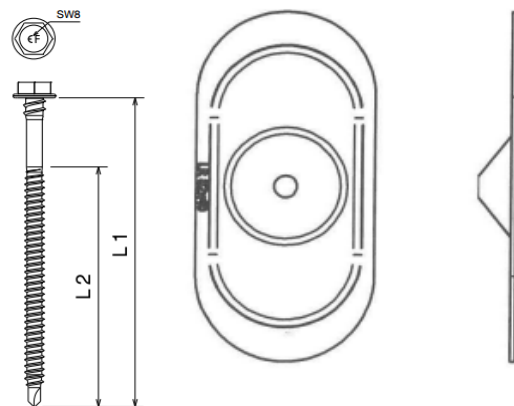
Fig. 2 – Vis LR ETANCO® EHB DF 2C + plaquette LR ETANCO® 82x40 R DF
