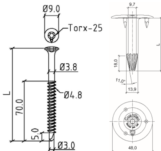
Fig. 7 – Vis AFAST GUARDIAN BS 48 + tube AFAST GUARDIAN RB 48
