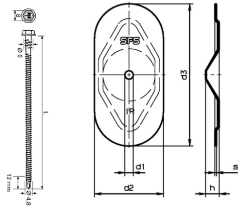
Fig. 1 – Vis SFS ISOFAST® IR2-S + plaquette SFS ISOFAST® IR 82x40
