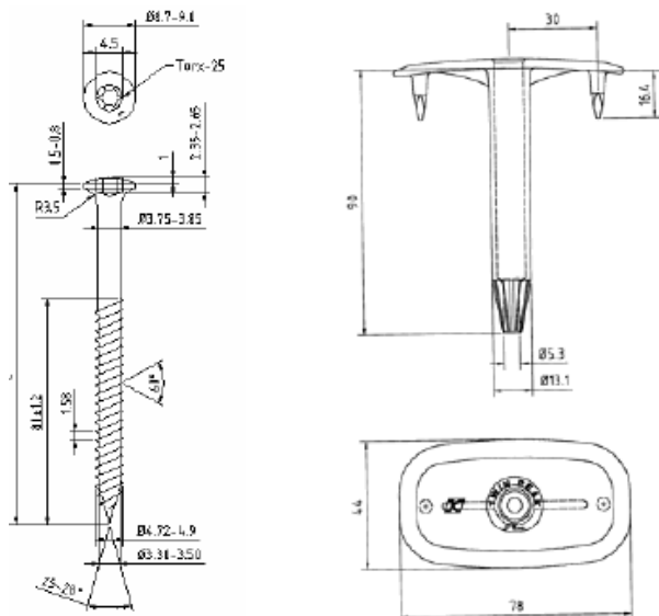
Fig. 3 – Vis SFS ISOTAK® PS-48 + tube SFS ISOFAST® TWIN PEAK PLUS
