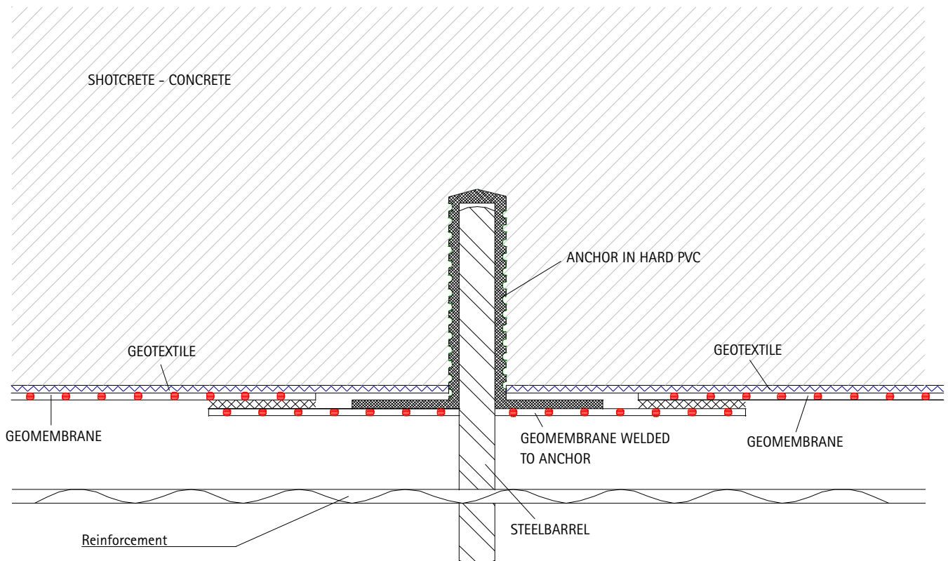
Watertight Hard PVC Anchor
