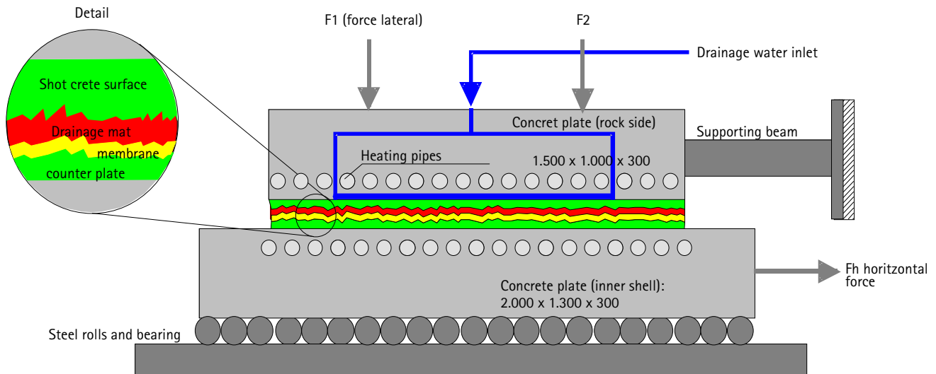
Figure7: Cross-section of the compression/shear set-up with heating and drainage capability, the top plate (fixed) corresponds to the shotcrete surface of the outer tunnel shell
